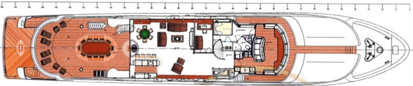
UPPER DECK
